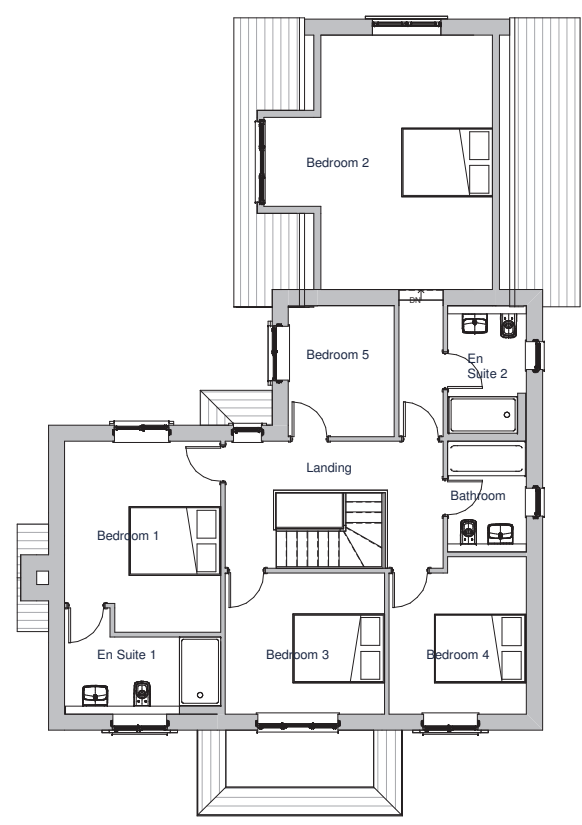
2 1.1 First Floor 1: 50
