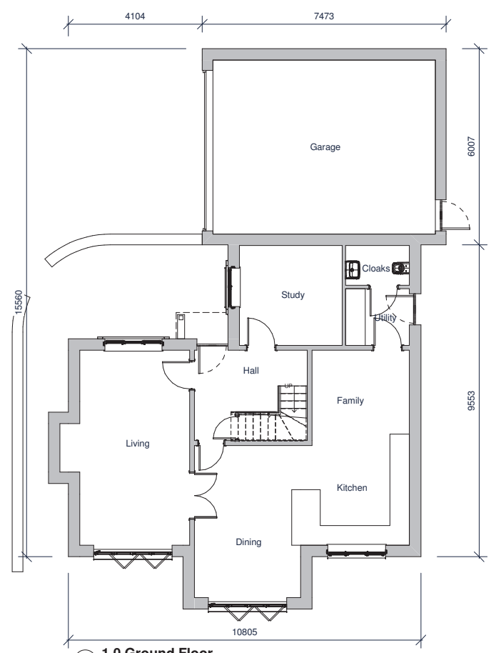
1 1.0 Ground Floor 1: 50
